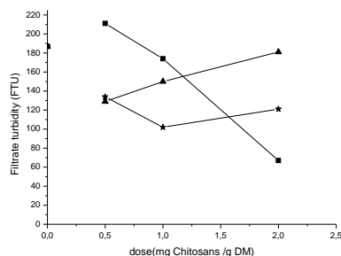
Figure 4. Variation of filtrate turbidity with chitosan dose for each flocculant RSDMDA7dT30 ( ★ ), RSDA7dT30 ( ▲ ) and ChitosCom ( ■ ).
