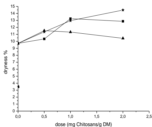
Figure 2. Variation of cake dryness with chitosan dose for each flocculant RSDMDA7dT30 (★), RSDA7dT30 (▲) and ChitosCom (■).
