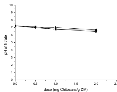
Figure 6. Variation of filtrate pH with chitosan dose for each flocculant RSDMDA7dT30 ( ★ ), RSDA7dT30 ( ▲ ) and ChitosCom ( ■ ).
