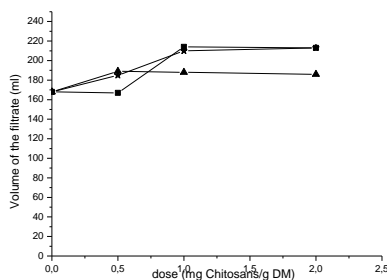
Figure 3. Variation of filtrate volume with chitosan dose for each flocculant RSDMDA7dT30 ( ★ ), RSDA7dT30 ( ▲ ) and ChitosCom ( ■ ).
