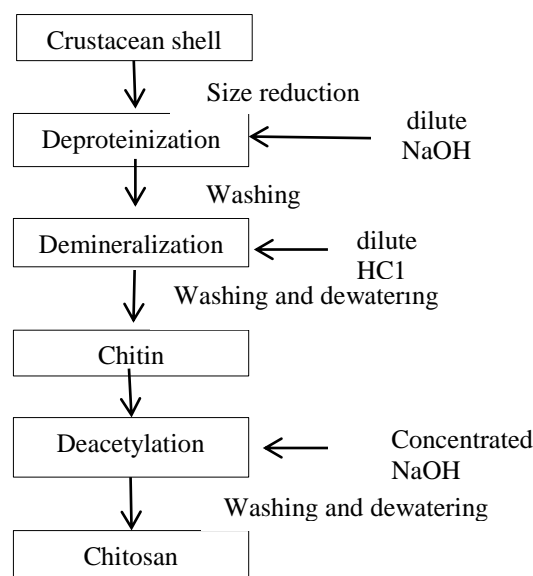
Figure 1. Conventional diagram of chitin and chitosan processing [4].
