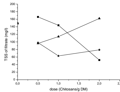
Figure 5. Variation of filtrate suspension matter with chitosan dose for each flocculant RSDMDA7dT30 ( ★ ), RSDA7dT30 ( ▲ ) and ChitosCom ( ■ ).
