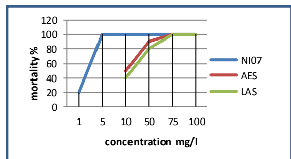
Figure5. Comparison ecotoxicity of three surfactants
