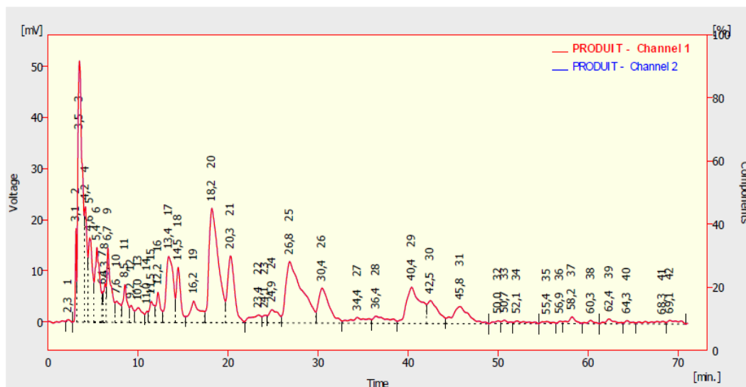
Figure 1. Chromatogram of surfactants
