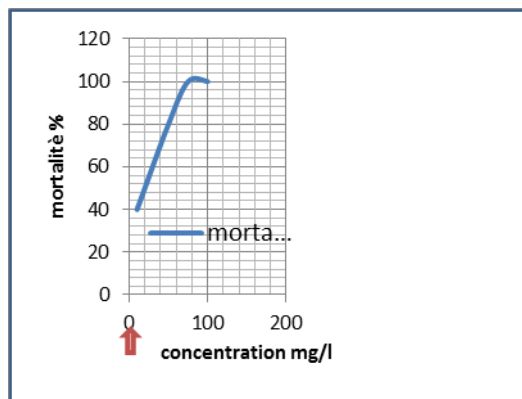
Figure 2. Mortality of mussels on function concentration of LAS
