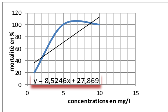
Figure 3. Mortality of mussels on function concentration of NI O7
