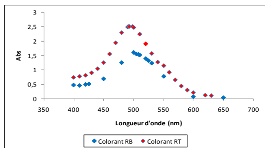
Figure 4. Determination of the maximum wavelength of the two dyes RT and RB
