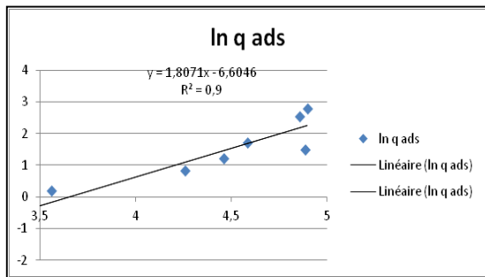
Figure 6. Application of Freundlich model to RB-zincophosphate system.
