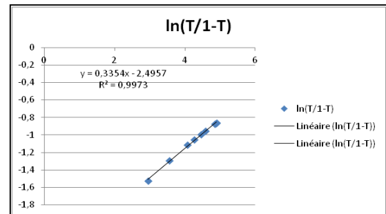
Figure 7. Fit of Sips model on the RB-zincophosphate system.
