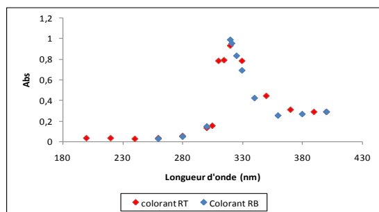
Figure 4. UV-visible spectra of the two dyes RT and RB: determining the cyclical nature.
