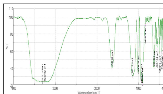
Figure 3. IR spectrum of the new zincophosphate-methionine.
