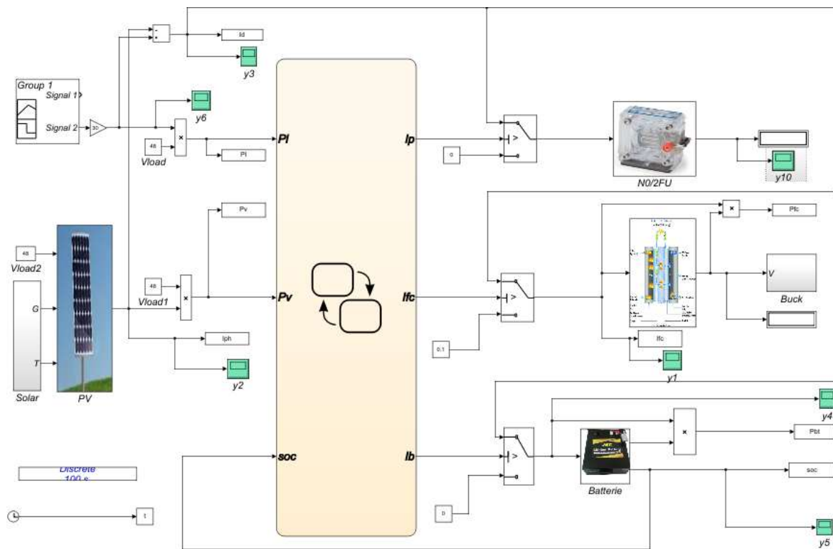
Figure 5. SIMULINK controller schematic
